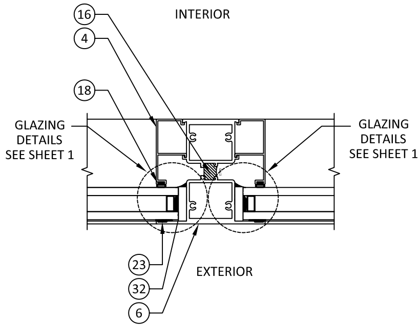
C 6 HORIZONTAL SECTION MEETING RAIL FX-FX ( MAX SPAN 72" )
