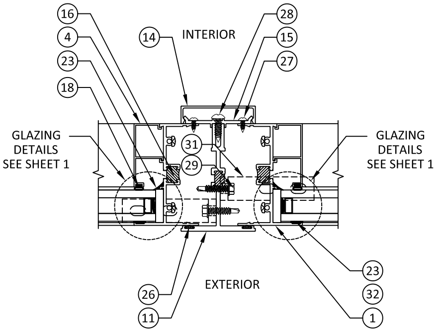
B 6 HORIZONTAL SECTION MULLION ( SPAN UP TO 72" )
