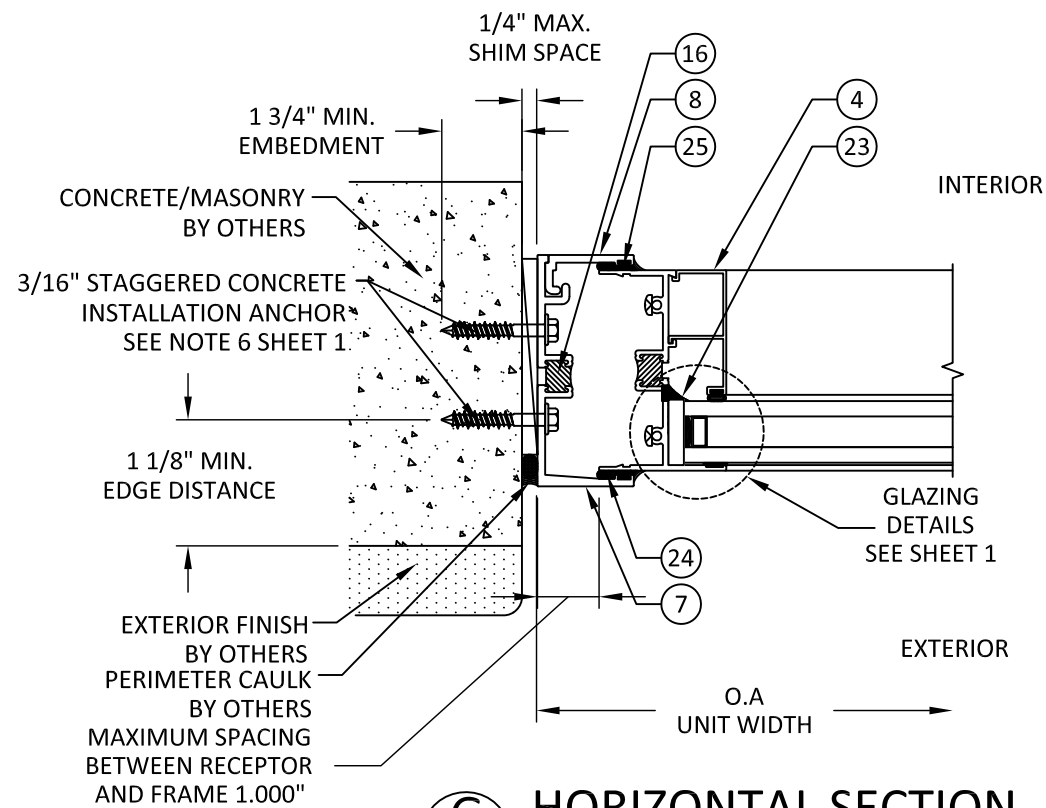
G 5 HORIZONTAL SECTION JAMB - CONCRETE OR CMU THROUGH FRAME INSTALLATION
