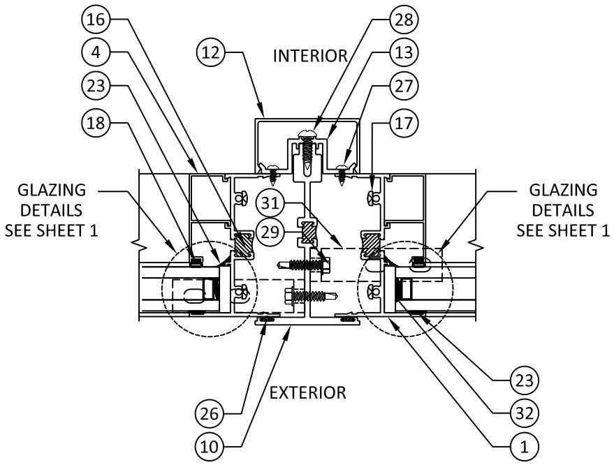
A 6 HORIZONTAL SECTION MULLION ( SPAN ABOVE 72" )
